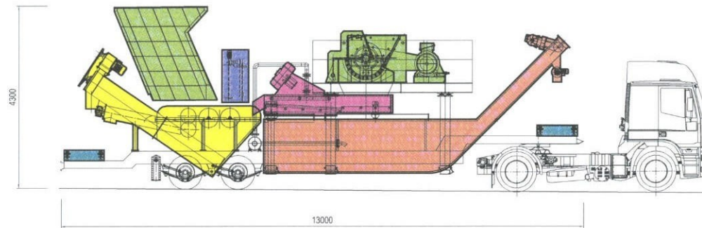
BREAKER ON TRAVEL - TRAILER 1
